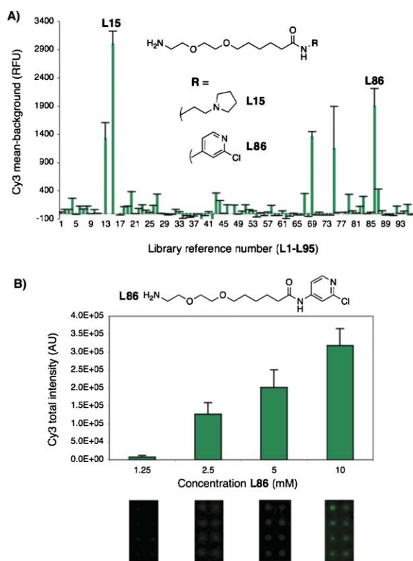
Fig. 3 A) Library-CarR small-molecule microarray screening results of the library reference number versus the background corrected Cy3 mean intensity value (based on the average across 4 replicate spots per ligand). Potential binders were selected based on having a signal-to-noise ratio (SNR) higher than 3 (the lower limit for detection), which included L15 & L86 . L77 was removed for clarity due to auto-fluorescence. B) Background corrected Cy3 total intensity (based on the average across 8 replicate spots per concentration) versus concentration of L86 and the corresponding Cy3 images. Error bars for both charts correspond to the standard deviation, RFU = relative fluorescent units, AU = arbitrary units. See ESI† for other scans and plots.
