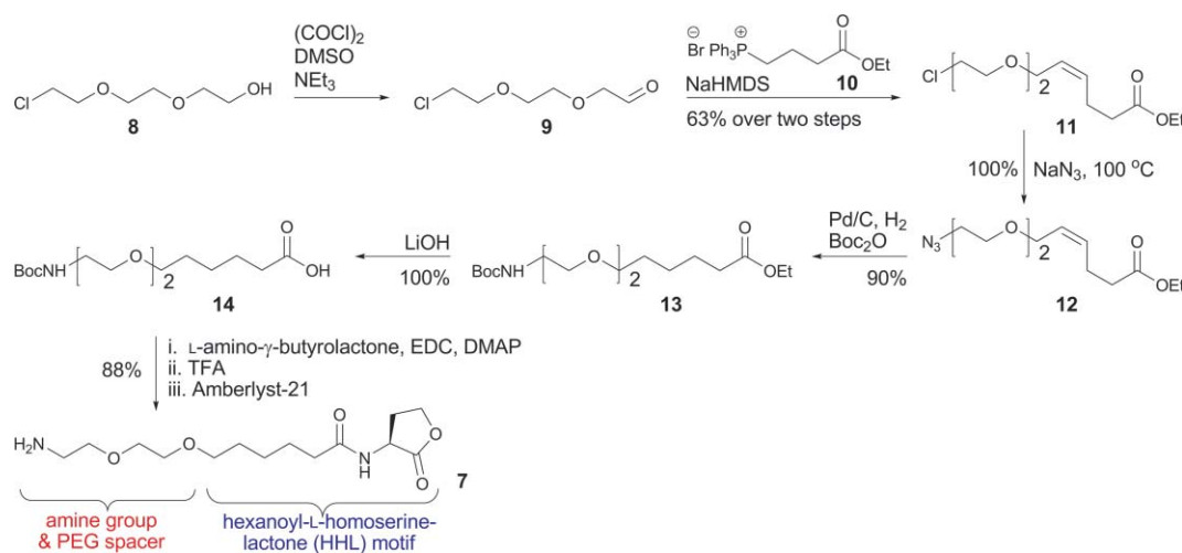
Scheme 1 Synthesis of target AHL analog molecule 7 . PEG = polyethyleneglycol, DMSO = dimethoxy sulfoxide, NaHMDS = sodium bis(trimethylsilyl)amide, TFA = trifluoroacetic acid, Boc = tert -butoxycarbonyl, EDC = 1-(3-dimethylaminopropyl)-3-ethylcarbodiimide hydrochloride & DMAP = dimethylaminopyridine.
