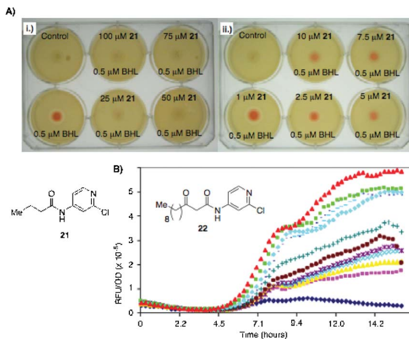
Fig. 6 A) Phenotypic assay of carbapenem production in Serratia sp. ATCC39006. Wells contained a lawn of carbapenem sensitive E. Coli and the inoculated Serratia sp. ATCC39006 mutant called LIS, which is unable to produce BHL and the indicated concentration of its native quorum sensing ligand BHL. Activation of carbapenem production is observed by the generation of a halo in the E. coli overlay at 0.5 \mu\text{M} BHL in well 6 of plate i. Carbapenem production was inhibited by the additional presence of the 2-chloro-pyridine BHL analogue 21 from 10–2.5 \mu\text{M} . B) Quorum sensing antagonist ( \text{IC}_{50} ) determination in P. aeruginosa by suppression of gfp production in the MH602 strain. \text{IC}_{50} for 22 = 10–20 \mu\text{M} . Concentrations of 22 : \blacklozenge 166 \mu\text{M} , \blacksquare 83 \mu\text{M} , \blacktriangle 42 \mu\text{M} , \times 21 \mu\text{M} , \ast 10 \mu\text{M} , \bullet 5 \mu\text{M} , + 2.6 \mu\text{M} , - 1.3 \mu\text{M} , - 0.6 \mu\text{M} , \blacklozenge 0.3 \mu\text{M} , \blacksquare 0.2 \mu\text{M} , \blacktriangle Control.
