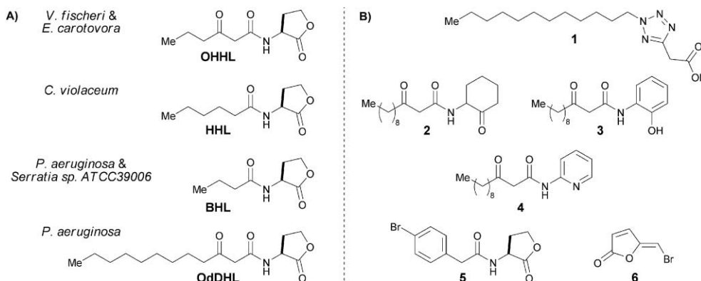
Fig. 1 A) N -acyl-homoserine lactones (AHL) used by Gram negative bacteria. B) Inhibitors of quorum sensing in P. aeruginosa . OHHL = 3-oxohexanoyl-l-homoserine lactone; HHL = hexanoyl-l-homoserine lactone; BHL = butanoyl-l-homoserine lactone; OdDHL = 3-oxododecanoyl-l-homoserine lactone.
