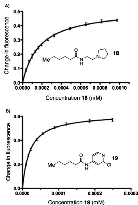
Fig. 4 CarR fluorometric ligand binding assays. The relative change in fluorescence was plotted against concentration using the Graphpad Prism software with a single binding site model. A) CarR- 18 K_d = 181 \mu\text{M} \pm 5.0 . B) CarR- 19 K_d = 21 \mu\text{M} \pm 0.4 . Excitation wavelength 292 nm, emission 335 nm & T = 30^\circ\text{C} . Error bars correspond to standard deviation across three replicate experiments. See ESI† for OHHL and 20 binding curves with CarR and EccR.
