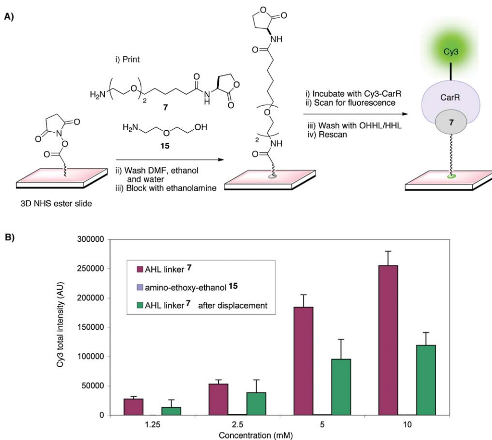
Fig. 2 A) Outline of the small-molecule microarray experiment between the immobilized AHL analog 7 and the protein CarR. The AHL analog 7 and the amino-ethoxy-ethanol control 15 were printed at 10, 5, 2.5 & 1.25 mM concentrations onto a 3D NHS ester slide before washing, blocking and scanning. For the displacement assay, the slide was washed with a solution containing native quorum sensing ligands OHHL and HHL before rescanning. Scanned images can be found in the ESI†. B) The background corrected Cy3 total intensities (based on the average across 8 duplicate spots) were plotted against the concentration of 7 and 15 . Error bars correspond to the standard deviation.
