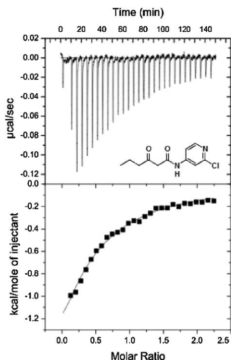
Fig. 5 ITC trace and binding isotherm for the injection of ligand 20 into CarR. [CarR] = 0.031 mM and [20] = 0.4 mM. T = 30\text{ }^\circ\text{C} , \Delta G = -6.8\text{ kcal mol}^{-1} , \Delta H = -1.4\text{ kcal mol}^{-1} , -T\Delta S = -5.4\text{ kcal mol}^{-1} , K_d = 11.2 \pm 1.1\text{ }\mu\text{M} . Fitted to single binding site model, stoichiometry fixed to n = 1 based on OHHL binding.
